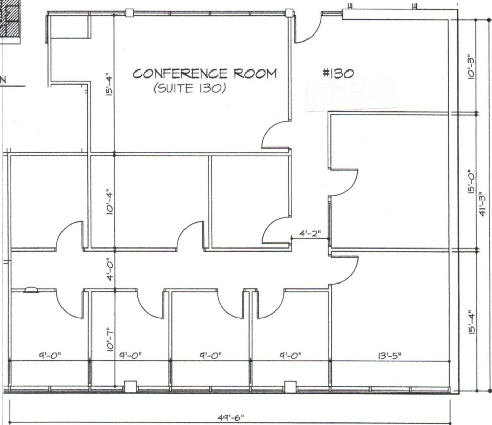
FLOOR PLAN 1/16" = 1'-0"
