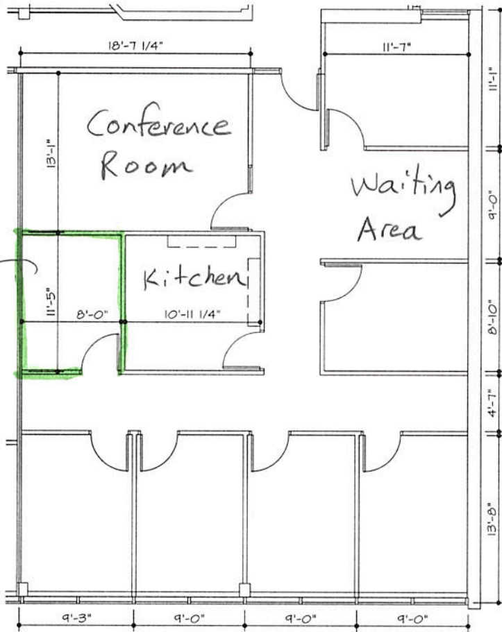
2 FLOOR PLAN 1/8"=1'-0"
